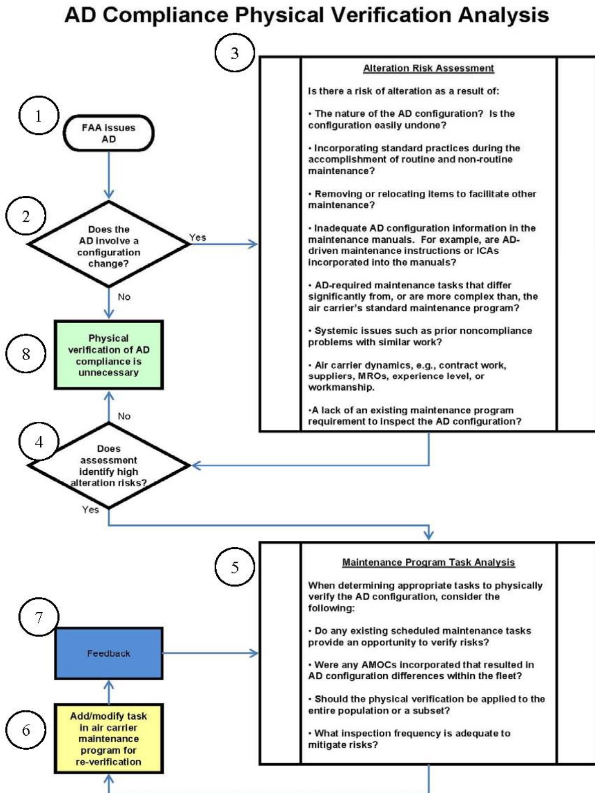
FIGURE 1. AIRWORTHINESS DIRECTIVE COMPLIANCE PHYSICAL VERIFICATION FLOW CHART
